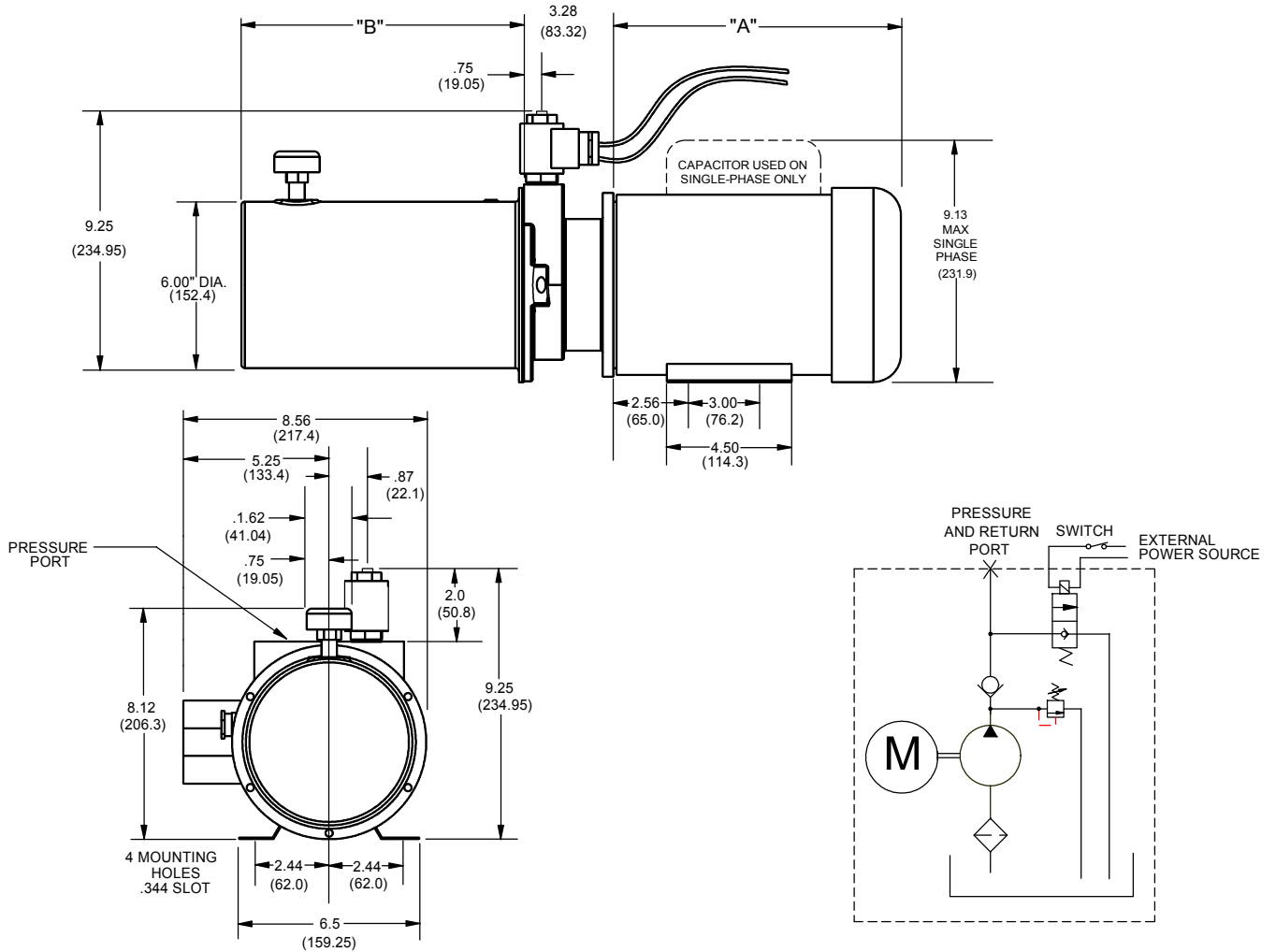
MOTOR DIMENSION CHART
